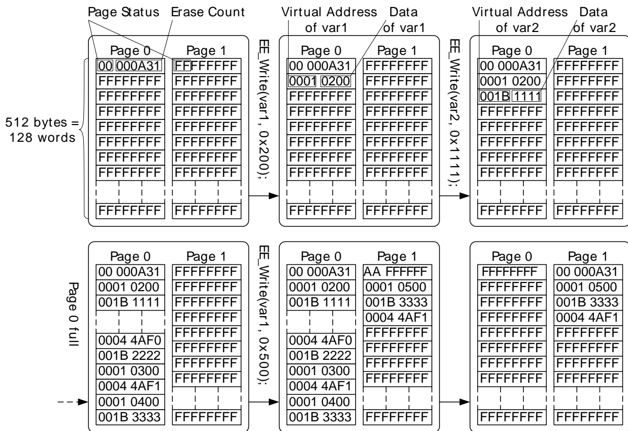
Figure 2.2. EEPROM Emulation Variable Flow.
